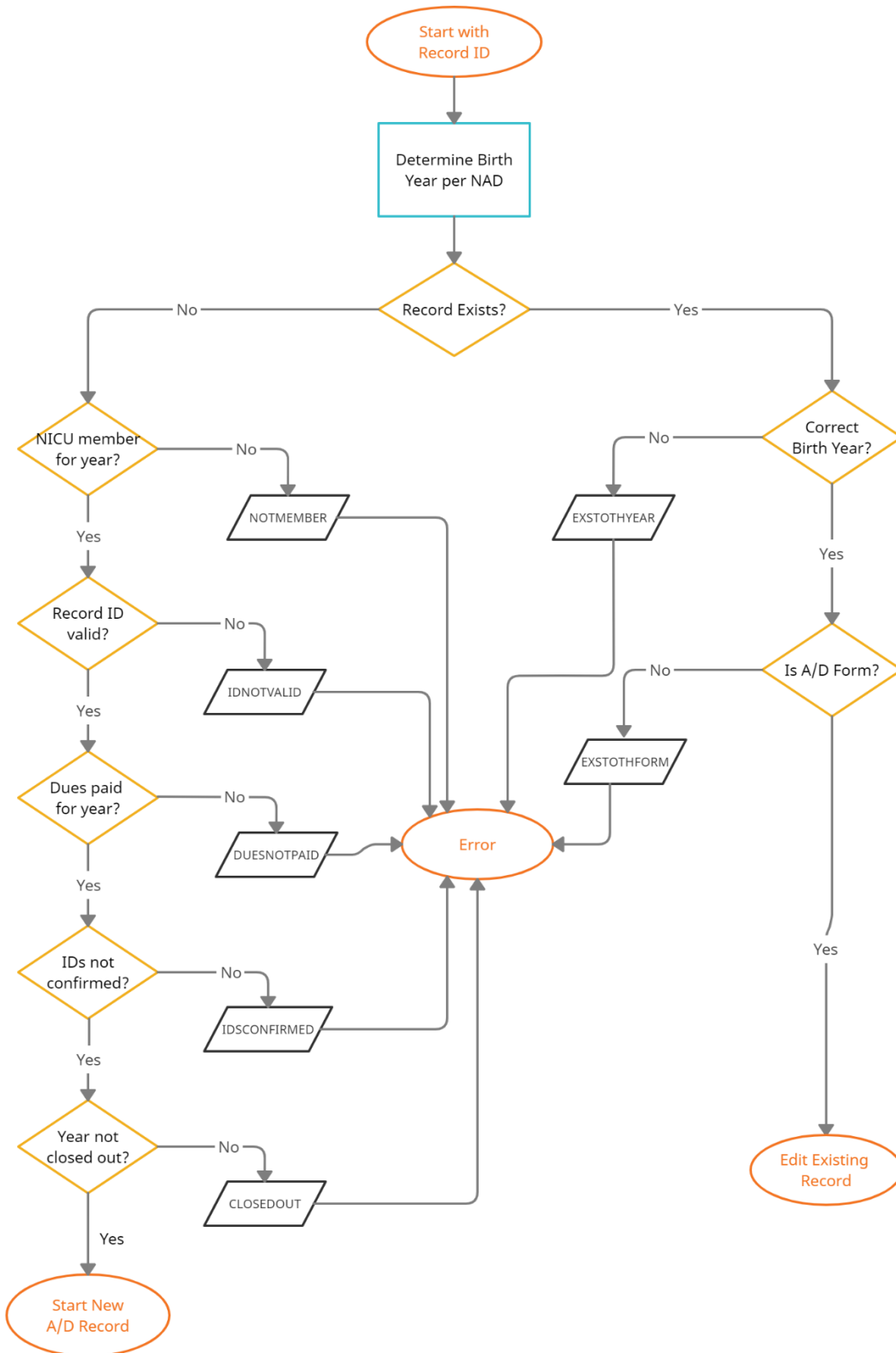
Figure 7: Flow Chart for Editing an Existing or Adding a New NICU A/D Record from the NAD
