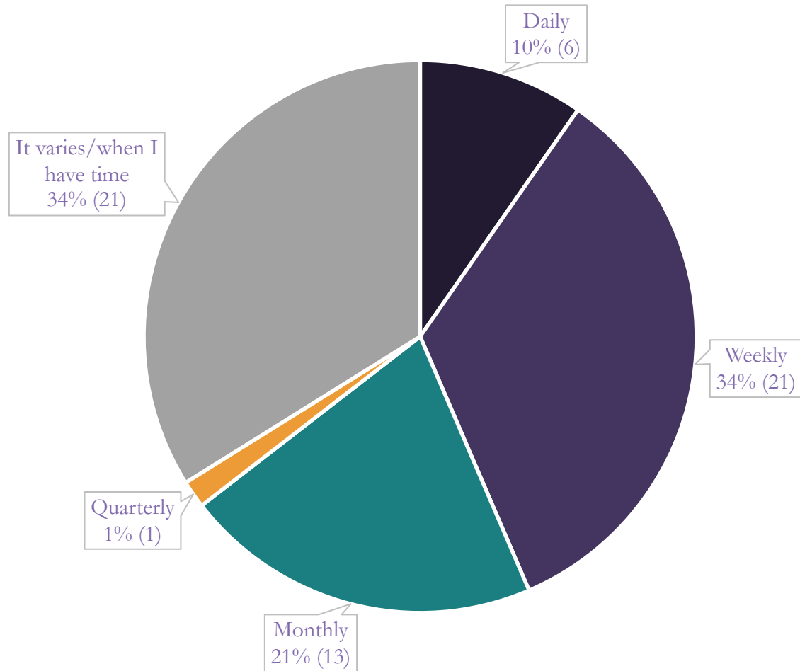
Abstract Data
