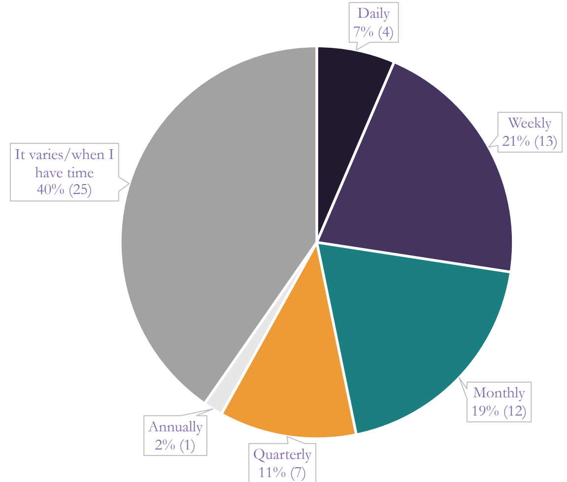
Enter Data
